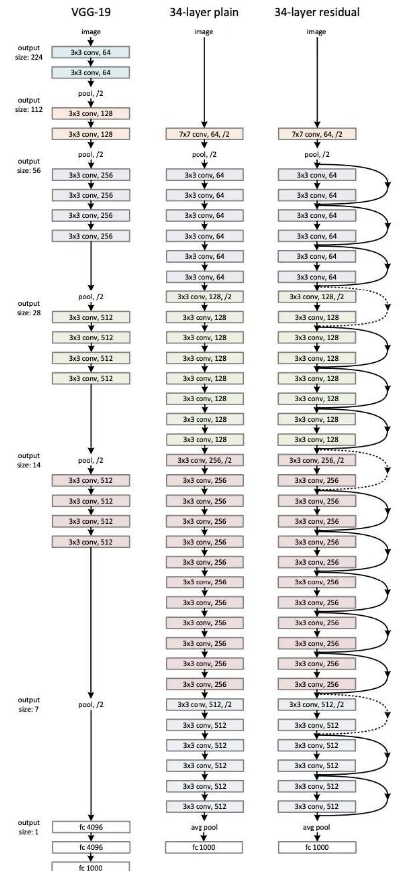
Figure 3. Example network architectures for ImageNet. Left: the VGG-19 model [41] (19.6 billion FLOPs) as a reference. Mid- dle: a plain network with 34 parameter layers (3.6 billion FLOPs). Right: a residual network with 34 parameter layers (3.6 billion FLOPs). The dotted shortcuts increase dimensions. Table 1 shows more details and other variants.
